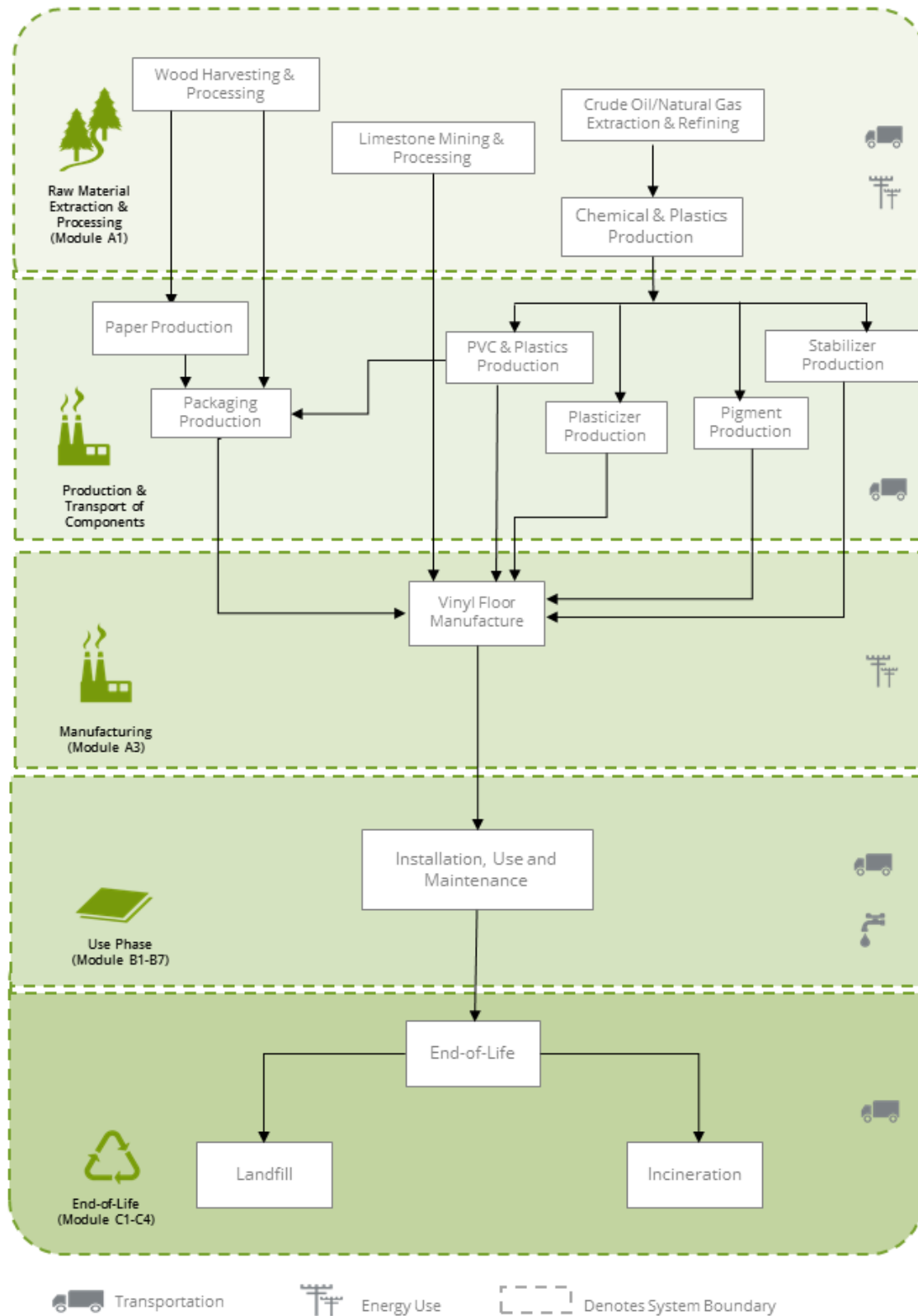
Figure 1. Flow Diagram for the life cycle of the VCT flooring product system.
